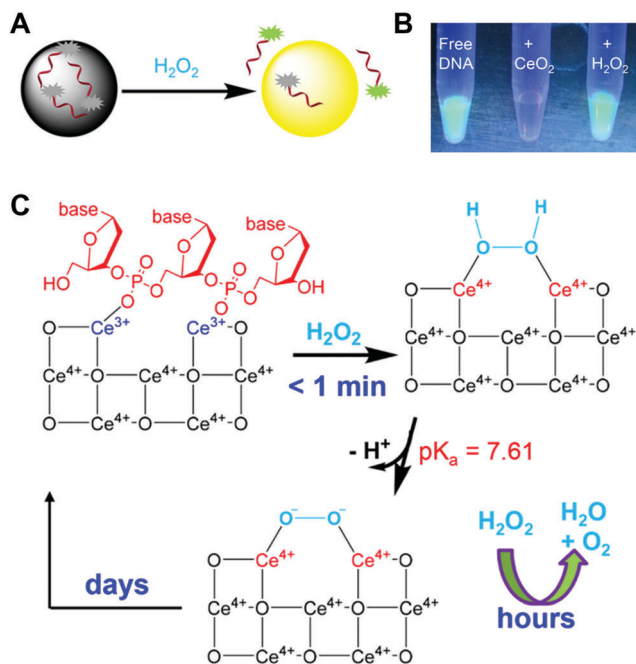
Fig. 28 (A) Sensing H 2 O 2 by displacing the adsorbed fluorescent DNA from the nanoceria surface. (B) A fluorescence photo of free FAM-A 15 DNA, after adding CeO 2 and then adding H 2 O 2 . (C) A proposed mechanism of H 2 O 2 induced DNA release by capping the nanoceria surface. Adapted with permission from ref. 831. Copyright (2015) American Chemical Society.
